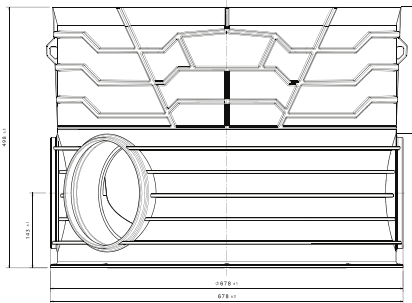
Technical drawing of straight through drain manhole 630/200
