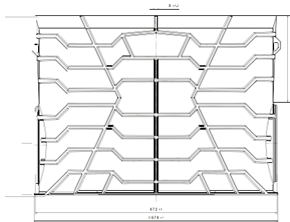
Technical drawing of straight through drain manhole 630/200
