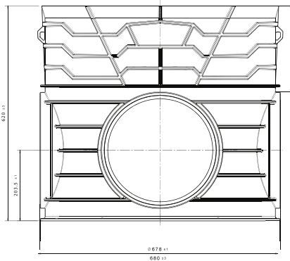
Technical drawing of straight through drain manhole 630/315
