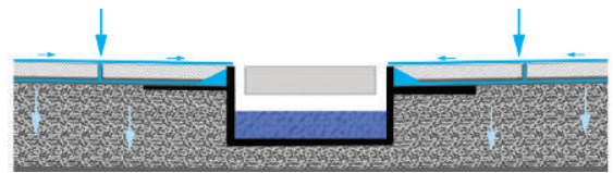
Cross section of linear drain
